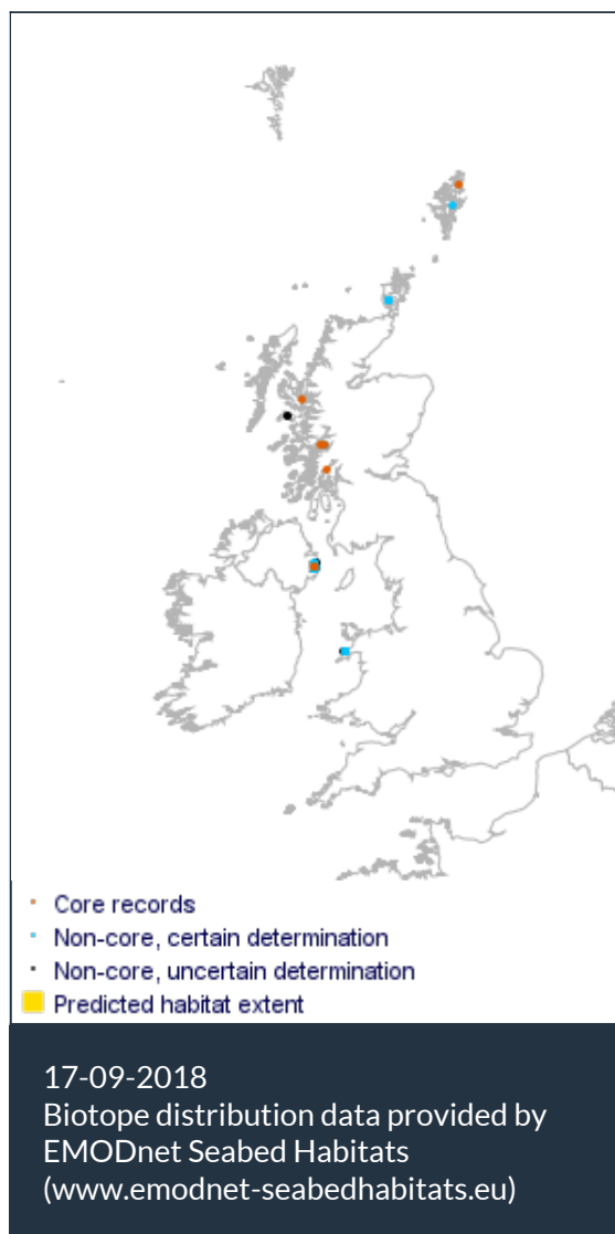
Modiolus modiolus beds with Chlamys varia , sponges, hydroids and bryozoans on slightly tide-swept very sheltered circalittoral mixed substrata Photographer: Keith Hiscock Copyright: Dr Keith Hiscock
